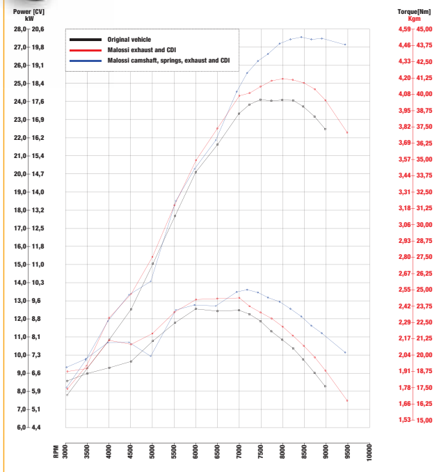
Power curve HONDA SH 300
